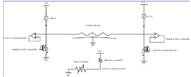
Figure 7 Analog Front-end
