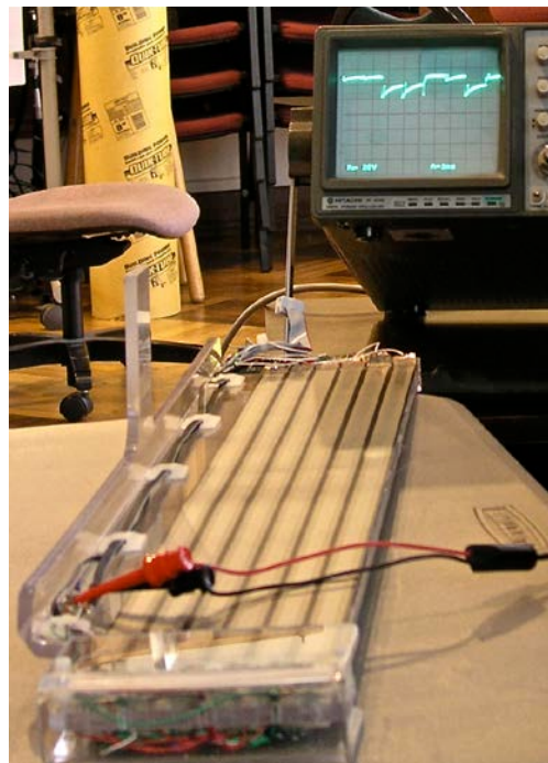
Figure 3. Fingerboard Array
