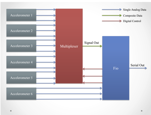
Figure 2: Overview of Data-Handling
