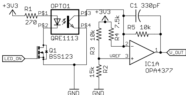
Figure 3: Schematic of optical reflectance sensors. Multiple sensors can be included on one op-amp channel by selectively activating each LED.
